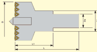
Note: Drill head complete with cartridges - Pilot Drill not included
